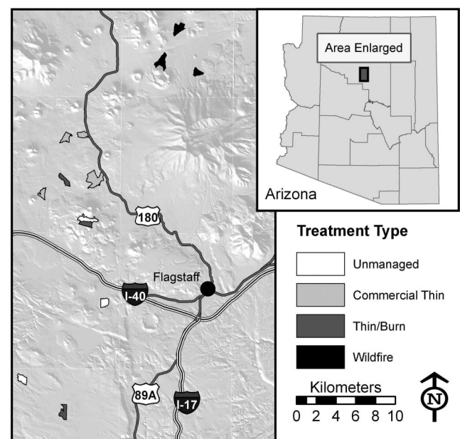
Figure 1. Locations of the unmanaged, commercially thinned, thinned and burned, and wildfire stand structural types in the Coconino National Forest near Flagstaff, Arizona, USA.
