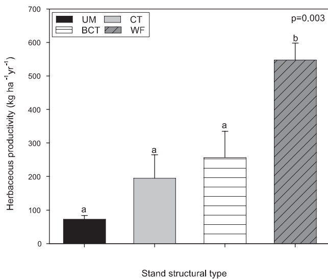
Figure 3. Mean aboveground herbaceous productivity across southwestern ponderosa pine stand structural types (UM, unmanaged; CT, commercially thinned; BCT, thinned and burned; WF, wildfire). Vertical lines denote 1 SEM. Means with different letters differed statistically ( P = 0.05 ).
