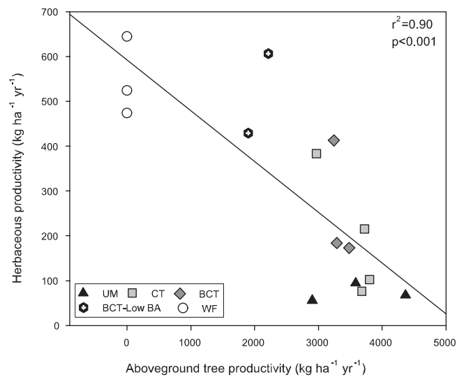
Figure 4. Relationship between 2005 aboveground herbaceous productivity and mean aboveground tree productivity across southwestern ponderosa pine stand structural types (UM, unmanaged; CT, commercially thinned; BCT, thinned and burned; BCT-Low BA, low basal area thinned and burned; WF, wildfire).
