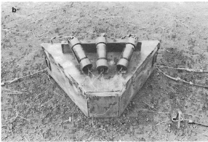
Figure 1. —Large (3-rocket), portable, rocket-net capture system as viewed from front (a) and rear (b). Note positioning of draglines and location of center anchor stake.
